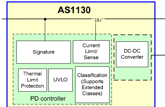
Figure 1: Top-Level Block Diagram of the AS1130
