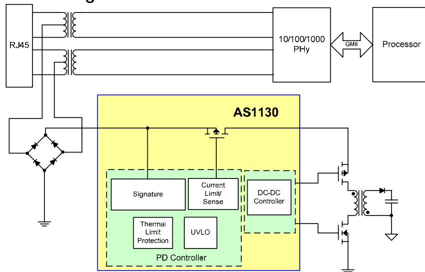
Figure 1, Typical Application Diagram for Gigabit Ethernet based PD (Flyback converter)
